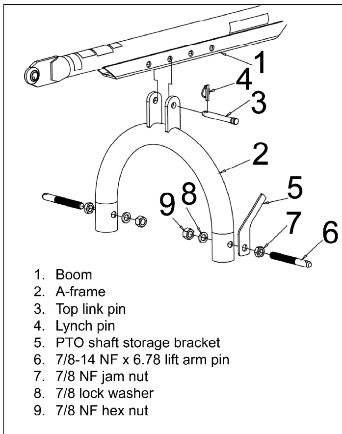
Figure 6. A-Frame to Boom Assembly
